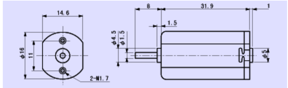
DN16 high speed type
