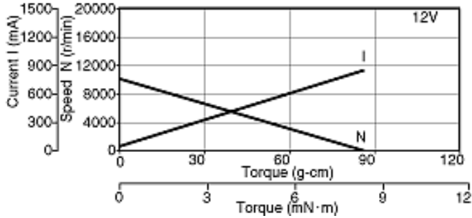
DN16 middle speed type
