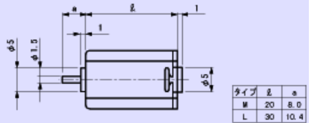
DN12 L type
